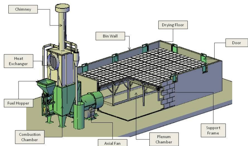
MAJOR COMPONENTS OF SIX-TON CAPACITY FLATBED GRAIN DRYER WITH BIOMASS FURNACE
